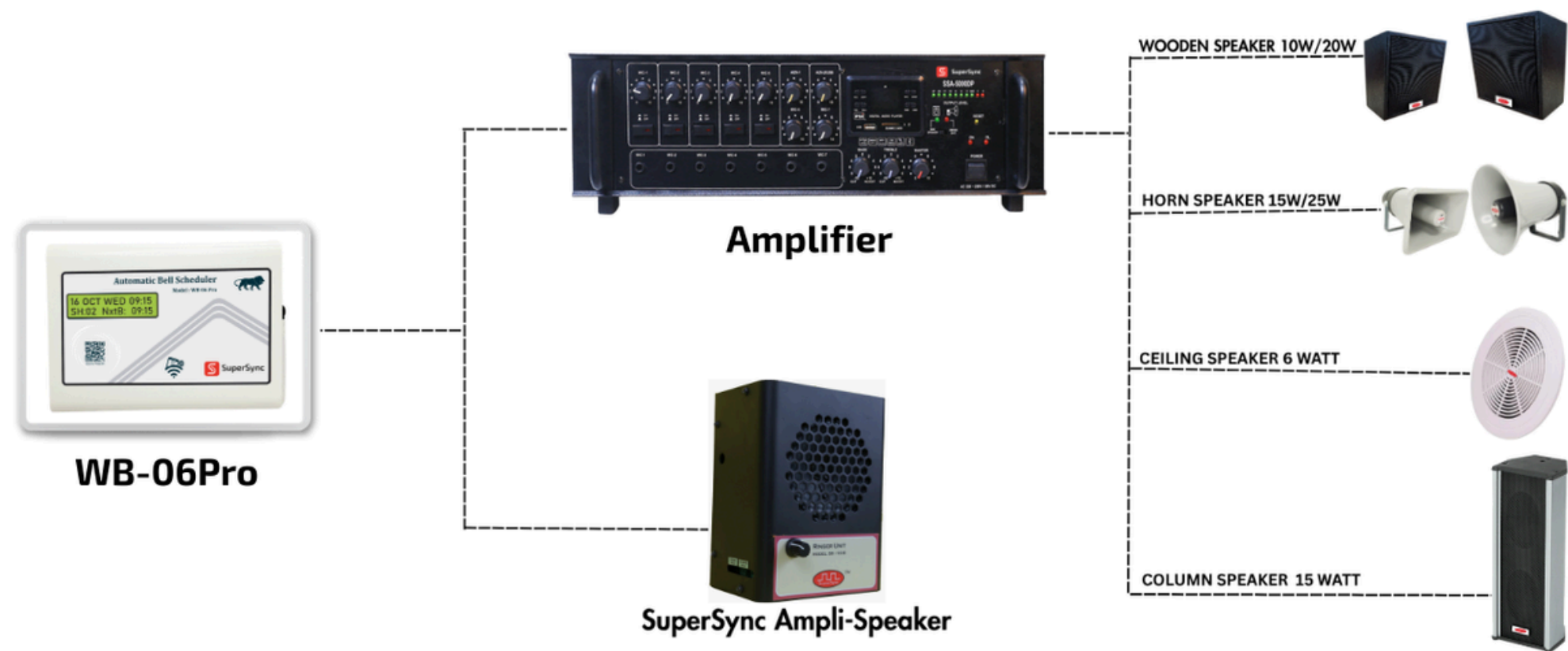
Connection Layout
